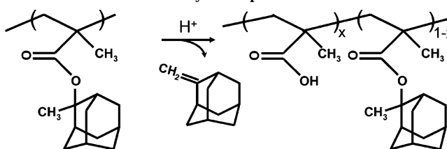
Scheme 2. Acid-Catalyzed Deprotection of PMAdMA
