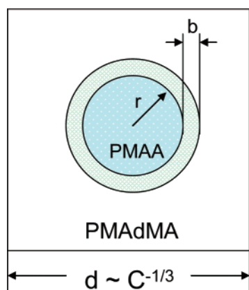
Figure 3. Schematic of the solid sphere model comprised of the core of radius r and shell of thickness b . The shaded region represents the PMAA domains produced by reaction. The boxed region corresponds to the average volume per photoacid related to the inverse photoacid concentration.
