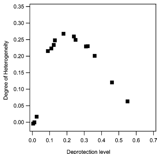
Figure 4. Degree of heterogeneity ( F_{\text{bond}} - 0.86\phi ) vs deprotection level in PMAdMA film for photoacid concentration C = 0.006 nm ^{-3} .
