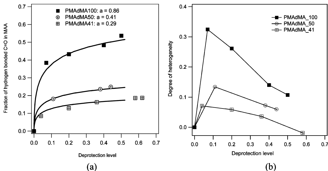
Figure 6. (a) Effect of comonomer composition on the hydrogen-bonded C=O fraction ( F_{\text{bond}} ) as a function of deprotection extent ( \phi ). (b) Degree of heterogeneity vs deprotection extent. The photoacid concentration is 0.007 nm -3 for all samples.
