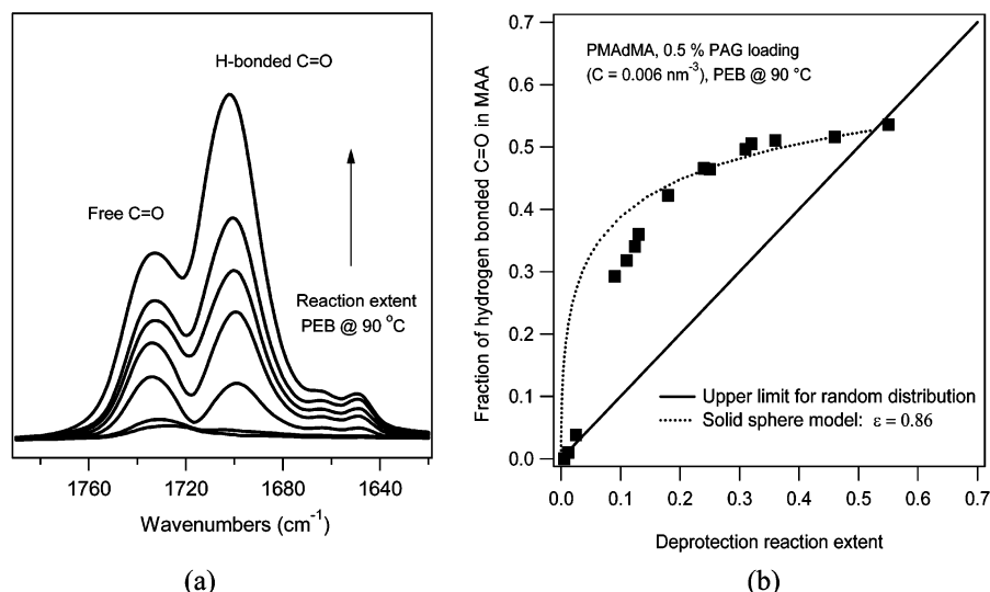
Figure 1. (a) Evolution of C=O stretching bands of MAA groups with reaction extent in PMAdMA samples. (b) Change of fraction of hydrogen-bonded C=O in MAA groups with deprotection reaction extent.
